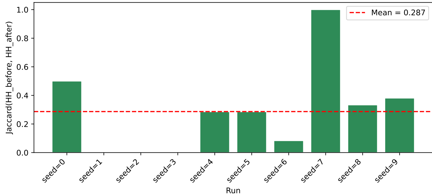
HH mask overlap: before vs after — ('german', 'isotonic')
